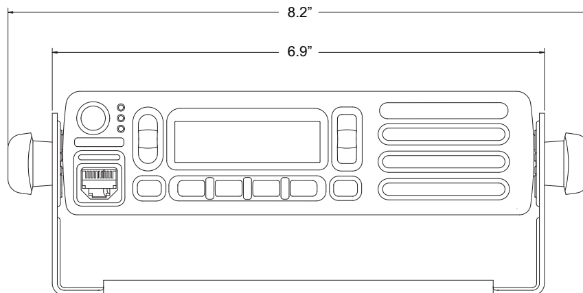
Figure 1-1 Front View of Dash Mount Trunion for MOTOTRBO CM200d/CM300d and XPR 2500 Mobile Radios
